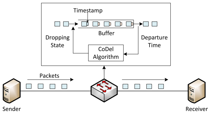
Fig. 18. CoDel scheme and algorithm. (1) CoDel uses timestamps to determine when a packet should be dropped. (2) The algorithm actively measures the queueing delay to determine if a packet will be dropped.
