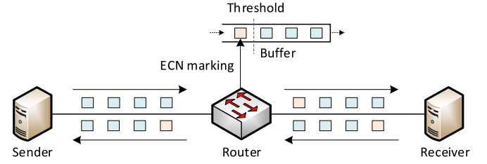
Fig. 9. ECN mechanism. The switch enables the ECN field in the packet header after the congestion surpasses a predefined threshold. Then, it notifies the sender that the network is experiencing congestion before the switch starts dropping packets.
