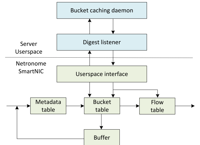
Fig. 26. System overview. OVS-CAB hardware offloading system consists of three principal components: (1) A P4-based hardware table pipeline that serves as the hardware data plane, (2) A userspace control plane module that implements OVS-CAB rule-caching logic, and (3) An RPC-based message system that communicates between the data plane and the control plane.
