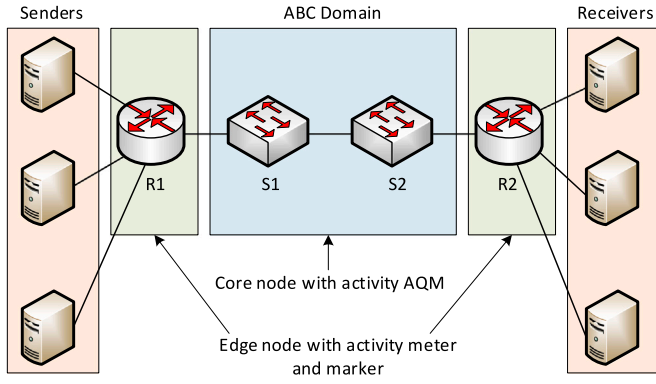
Fig. 19. Activity metering and marking are performed only by ingress nodes. Both ingress and core nodes apply activity AQM during packet forwarding.
