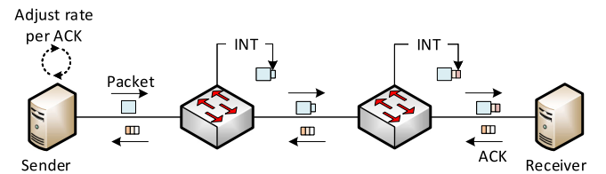
Fig. 12. HPCC: INT-based High Precision Congestion Control. Each switch adds telemetry data to the packets and piggybacked to the sender within the ACKs.
