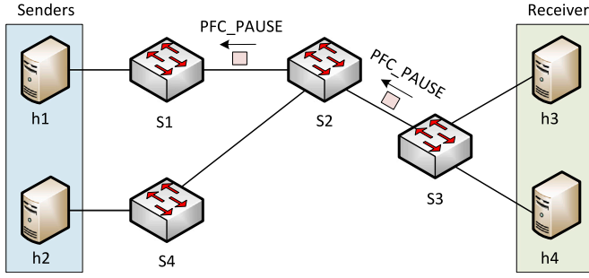
Fig. 15. Priority Flow Control (PFC) head-of-line blocking. An excessive queue length in switch S3 produce a PFC_PAUSE signal that will hold all the traffic passing through switch S2. P4QCN mitigates this issue by implementing an improved version of the QCN standard using P4 switches.
