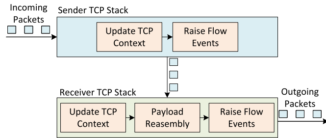
Fig. 27. Packet processing steps in mOS. Upon packets' arrival, mOS first updates its TCP context for the packet sender. Then, it sends the records of all flow events that must be triggered [144].
