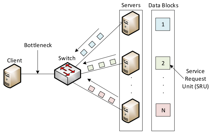
Fig. 6. A cluster-based storage environment. A client request data from multiple servers through synchronized reads. Then, the incoming packets cannot be handled by the switch. Thus, TCP suffers performance degradation [40].
