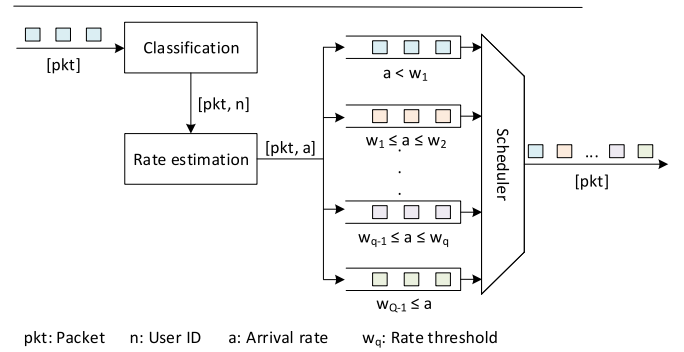
Fig. 21. FDPA forwarding pipeline scheme. Packets are classified on a per-user basis then, a rate estimator which measures the arrival bit-rate processes each packet according to a specific user. Packets are then stored in one of the Q priority queues. Finally, a strict priority (SP) scheduler serves queues in priority order (i.e., the lowest bandwidth first) [107].
