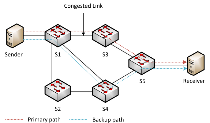
Fig. 14. Simplified Fast-TCP mechanism overview. The scheme has a primary path and many backup paths. Upon the failure, it evaluates the weight of the backup paths to reroute the traffic.
