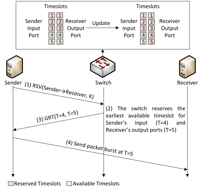
Fig. 16. PL2 algorithm [74]. The switch manages the reservations to avoid collisions. PL2 reduces end-to-end latency by proactively avoiding losses by implementing a protocol where the end host schedule a timeslot to start a data transfer.
