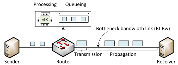
Fig. 17. Delay components: processing, queueing, transmission, and propagation delays. The queueing delay is the one that has a significant impact on TCP performance.
