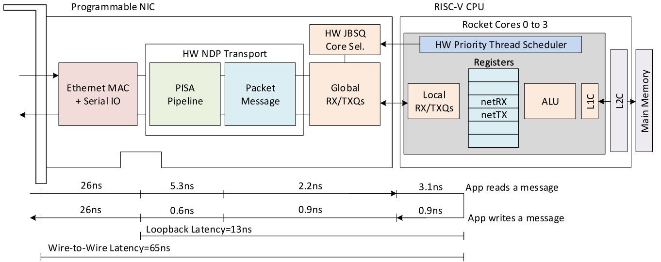
Fig. 25. The nanoPU design. The NIC includes ingress and egress PISA pipelines, a hardware-terminated transport, and a core selector with global RX queues; each CPU core is augmented with a hardware thread scheduler and local RX/TX queues connected directly to the register file. Total wire-to-wire latency is 65 ns [62].
