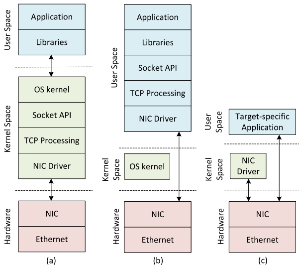
Fig. 23. Conventional and kernel bypassing OS architectures. (a) Conventional operating systems implement all network processing in the kernel space. (b) Kernel bypass architectures avoid overheads for kernel crossings by moving the protocol implementation into the application and providing applications with direct access to the NIC for sending and receiving packets [120]. (c) Hardware accelerated data-path architecture requires a target-specific application [121].
