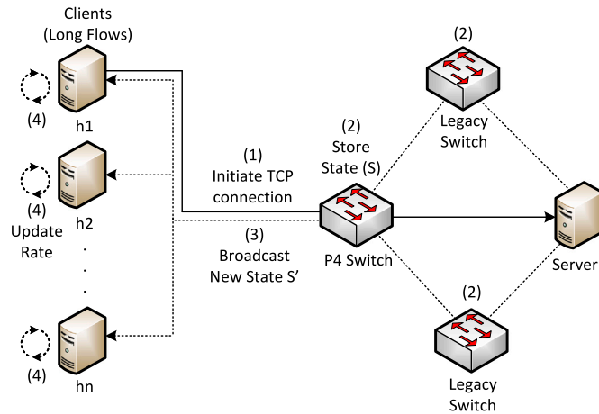
Fig. 11. High-level architecture of P4-enabled pacing system. The P4 switch identifies the number of TCP flows traversing it to notify the senders how to adjust the sending rate.
