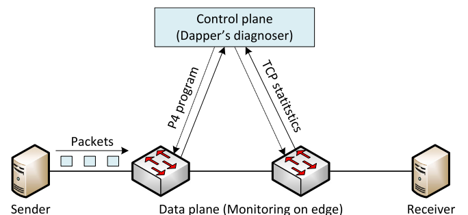
Fig. 29. Dapper's architecture : (1) Data plane monitoring on edge, (2) Control plane diagnosis techniques.
