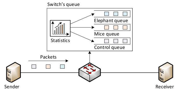
Fig. 10. Overview of the NCF mechanism. The authors categorized Internet traffic into two types: (1) Elephant flows, which involve the transfer of a large volume of data and has a long duration, and (2) Mice flows, which constitute flows with shorter duration and smaller data transfer sizes.
