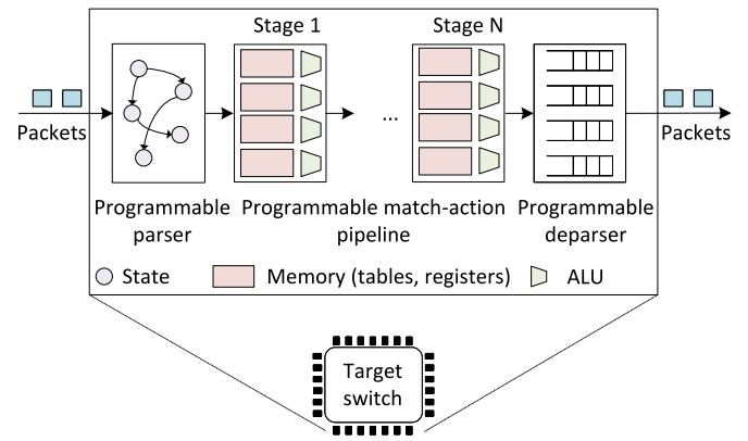
Fig. 2. The PISA architecture.
