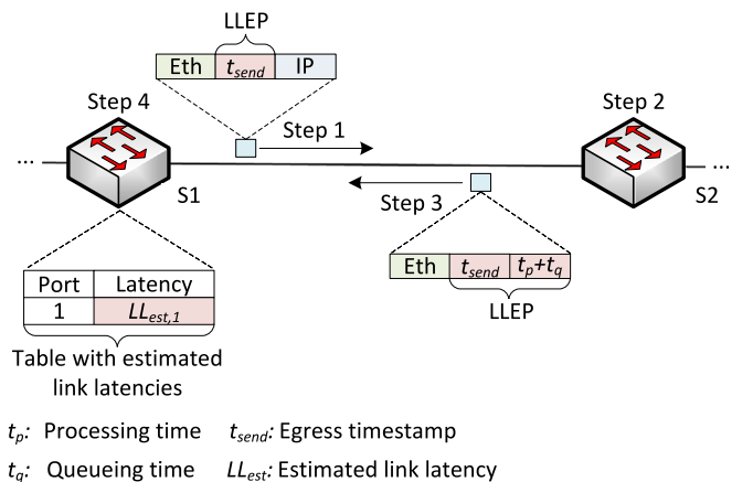
Fig. 22. Overview of the Link latency estimation protocol (LLEP) [108]. LLEP mitigates the lack of coordination among the clocks of the switches.
