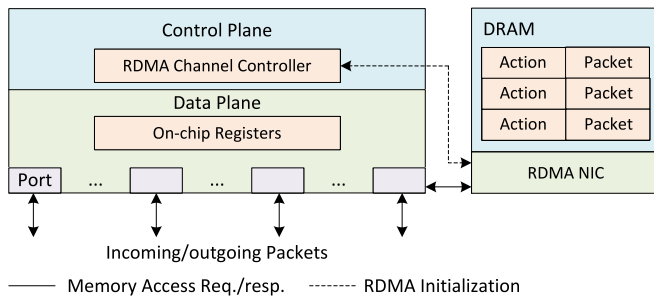
Fig. 35. External memory for data plane scheme. The data plane can utilize remote memory region registered RNICs by servers that are connected to the switch. The system comprises a remote lookup table, as an example. Other data structures can also be used [189].
