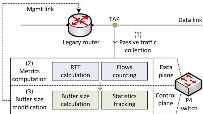
Fig. 33. High-level system overview. The P4 switch collects traffic and calculates the RTT per flow. Then, the P4 switch sets the buffer size of a legacy router [168].
