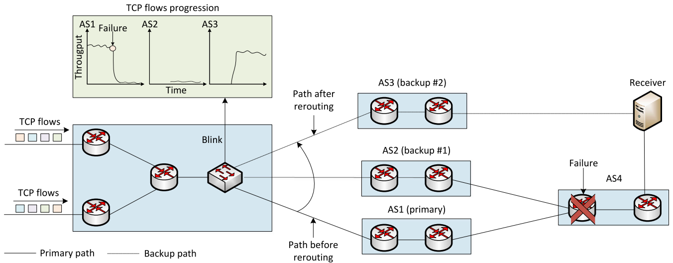
Fig. 28. Blink mechanism. Before the failure, the primary path is through AS1. Blink identifies the failure in AS4 measuring the retransmissions. Blink immediately reroutes TCP flows to both AS2 and AS3. The Blink switch determines that AS2 is not working and forwards all the traffic through AS3 [157].
