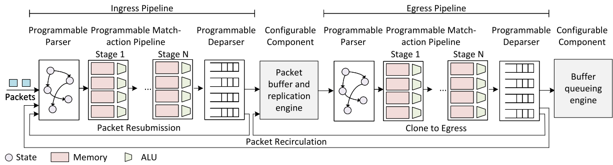
Fig. 3. Scheme of the Portable Switch Architecture (PSA) [25].
