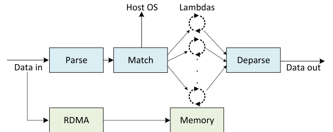
Fig. 24. \lambda -NIC's abstract machine model. \lambda s are independent programs that only a matching rule can invoke. The matching stage forwards the packets to the corresponding \lambda or the OS. The deparser associates the result of each \lambda to its corresponding header.
