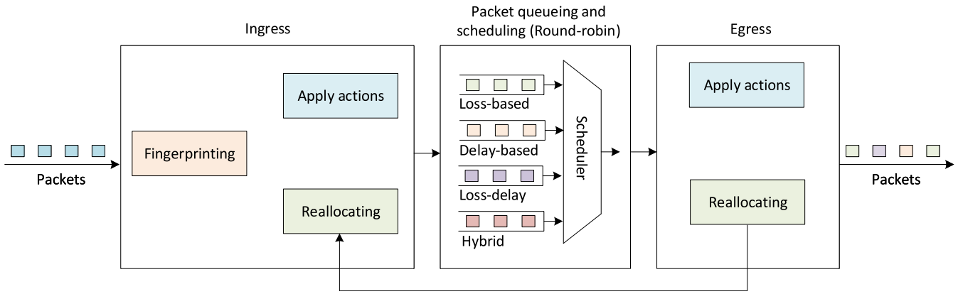
Fig. 13. The system comprises three modules: The fingerprinting module groups the flows according to their congestion control algorithm. The reallocation module redistributes the queues between groups when it is required, and the apply actions module applies custom policies to ensure fairness among flows [63].
